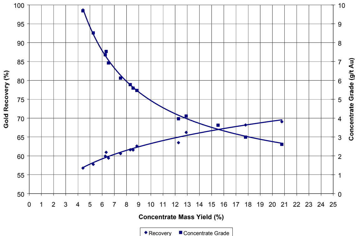
Figure 1. Kelsey Jig Performance – Recovery of Gold-containing Sulphides from CIP tailings
