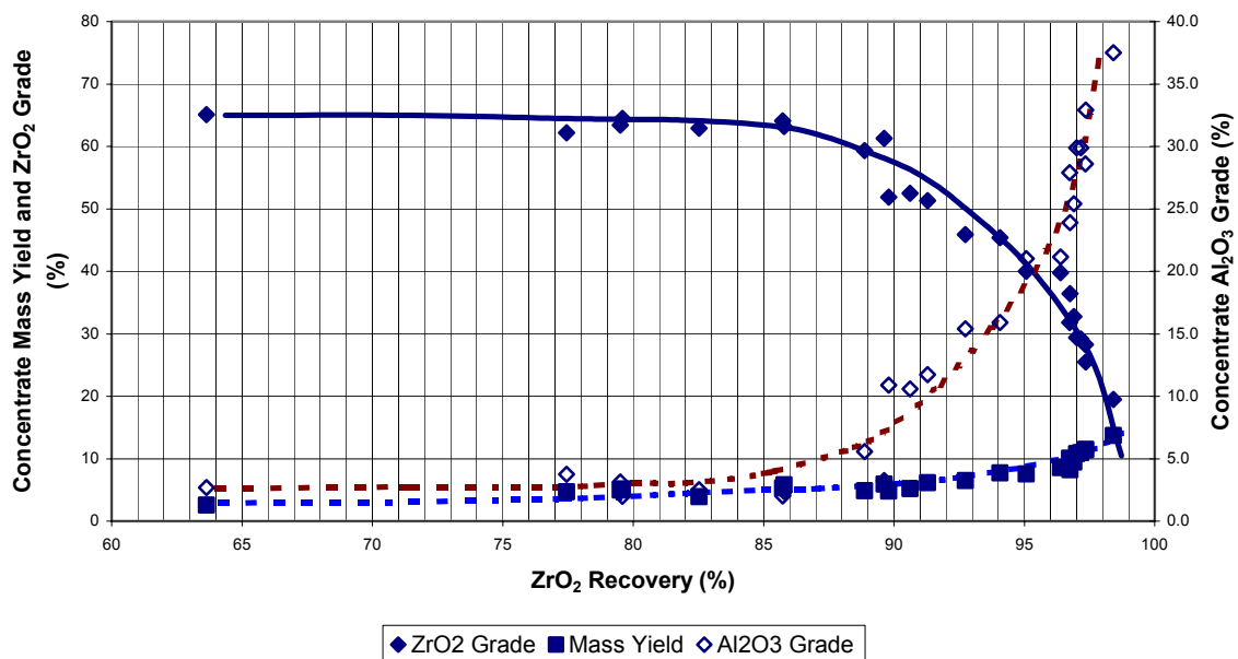
Figure 2. Kelsey Jig Performance – Separation of Zircon from Kyanite
