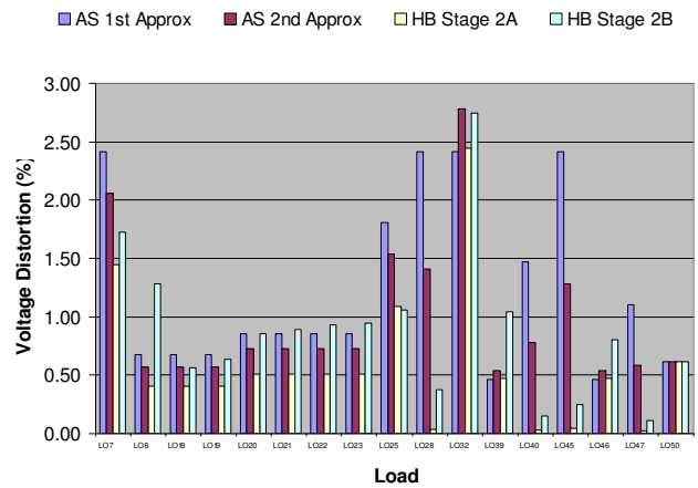
Graph 2: Emission Limits Derived from Current Harmonic Voltage Allocation Methods
