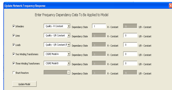
Figure 2: Example of API Interface
