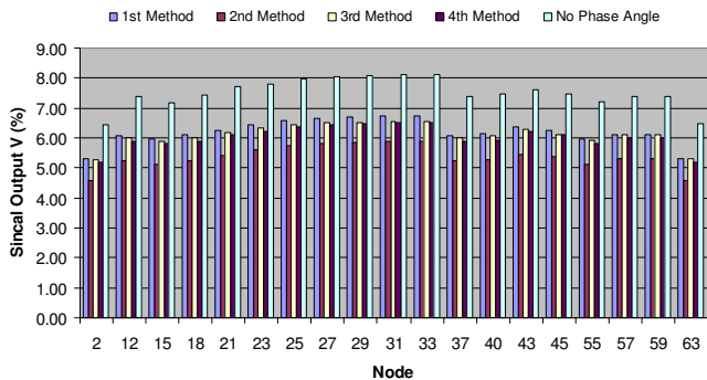
Graph 1: Sincal Derived Harmonic Voltage Distortion Levels Modelling All Loads with Phase Angle Distribution over 135°
